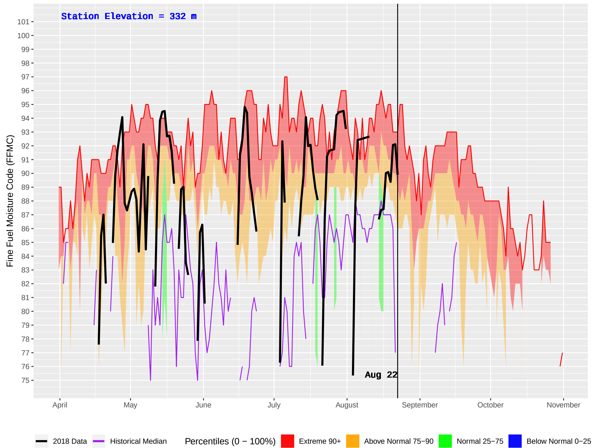
MACHMELL (101) : Historical (1990–2016) and Current (2018) Daily Fine Fuel Moisture Code (FFMC)
