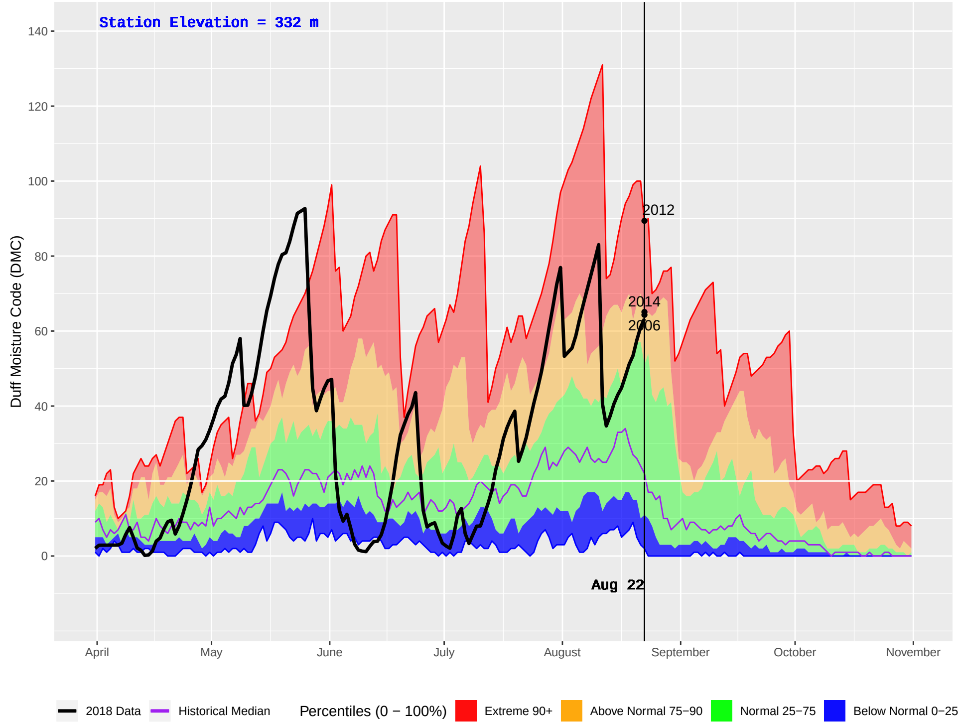
MACHMELL (101) : Historical (1990–2016) and Current (2018) Daily Duff Moisture Code (DMC)
