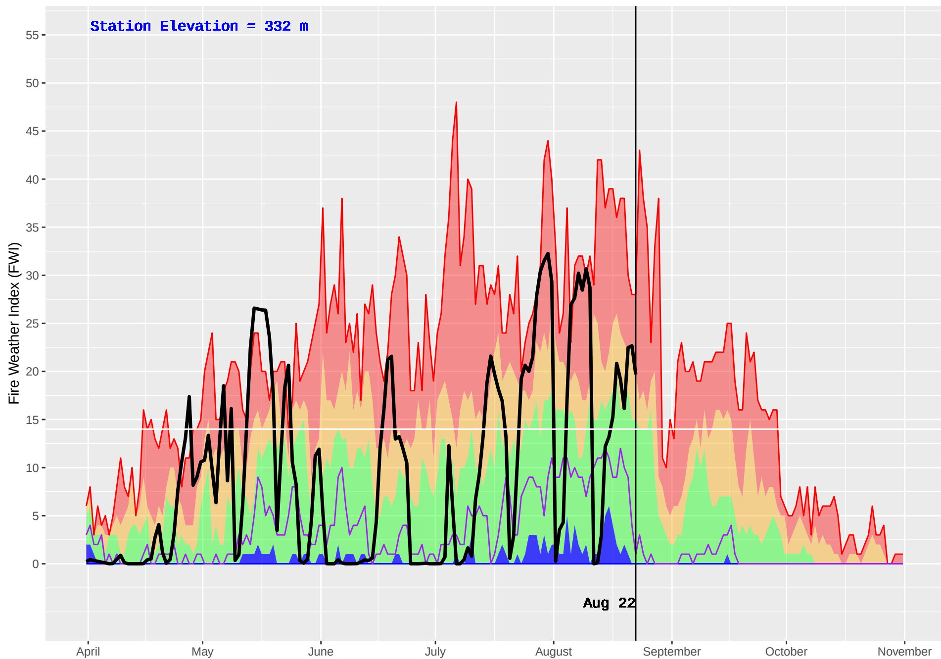
MACHMELL (101) : Historical (1990–2016) and Current (2018) Daily Fire Weather Index (FWI)
