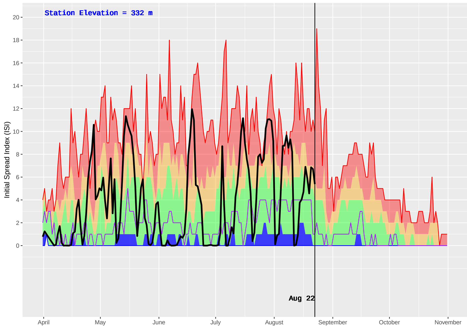
MACHMELL (101) : Historical (1990–2016) and Current (2018) Daily Initial Spread Index (ISI)
