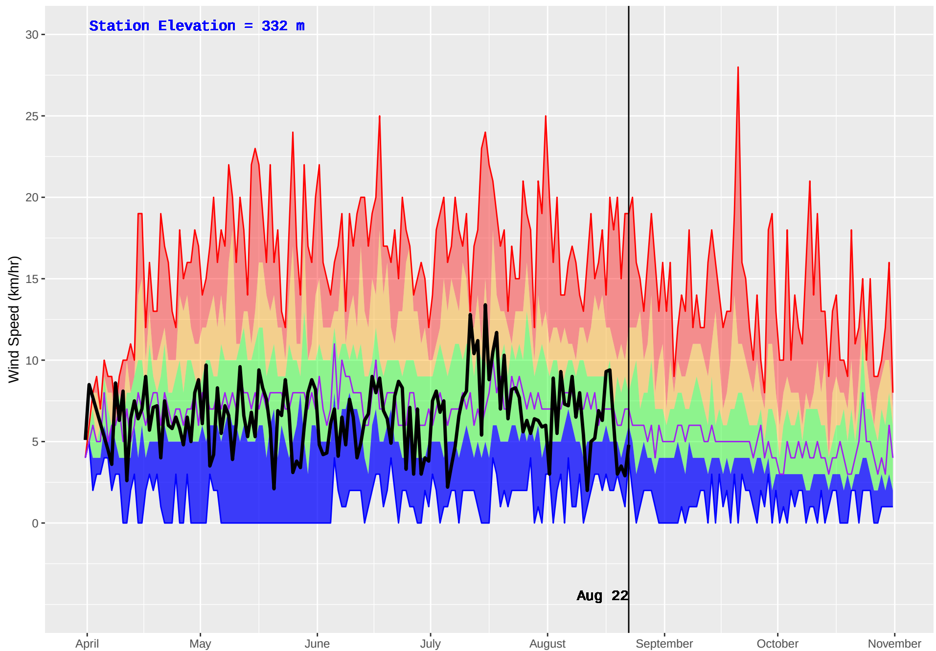
MACHMELL (101) : Historical (1990–2016) and Current (2018) Daily Wind Speed
