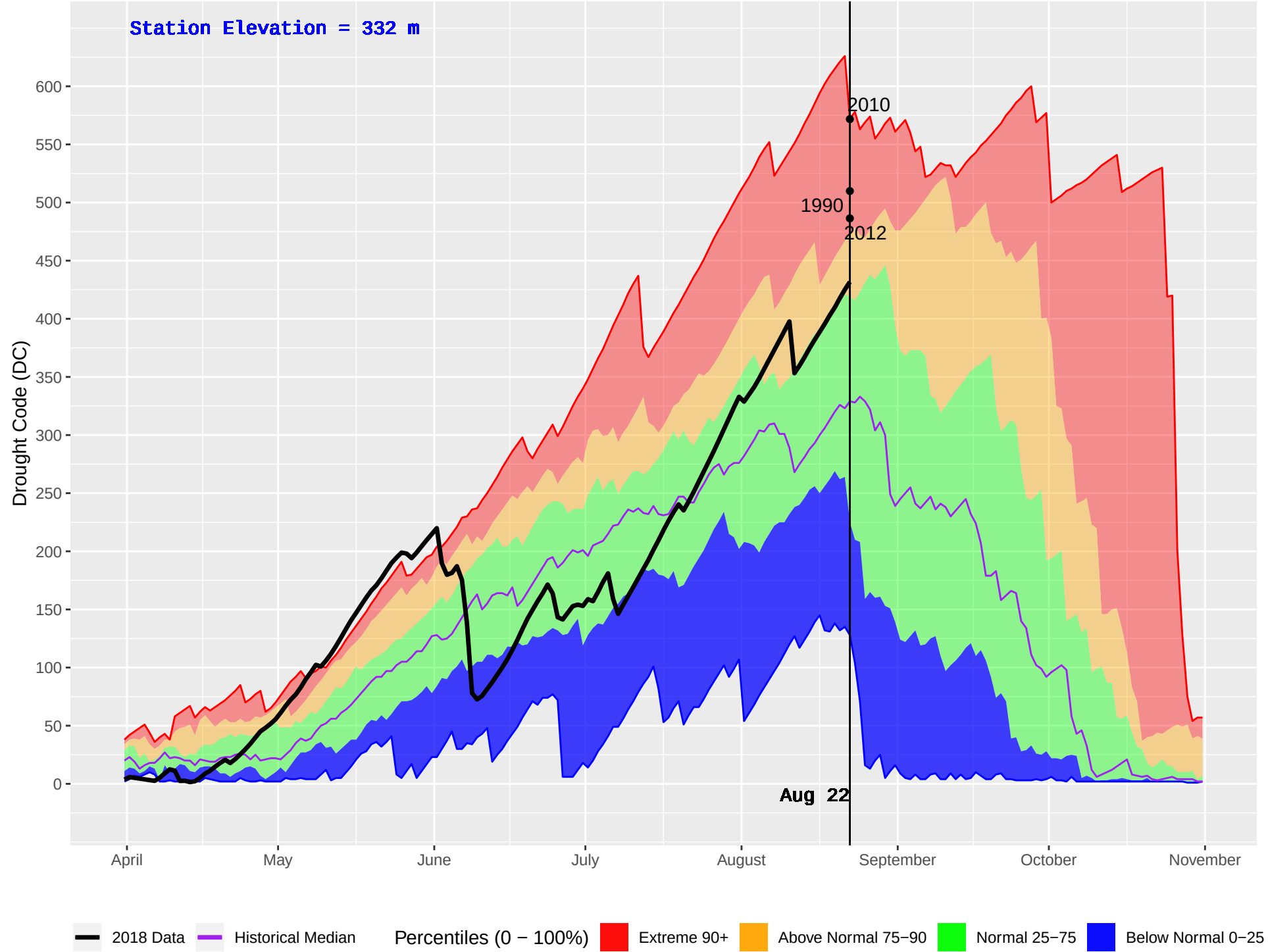
MACHMELL (101) : Historical (1990–2016) and Current (2018) Daily Drought Code (DC)
