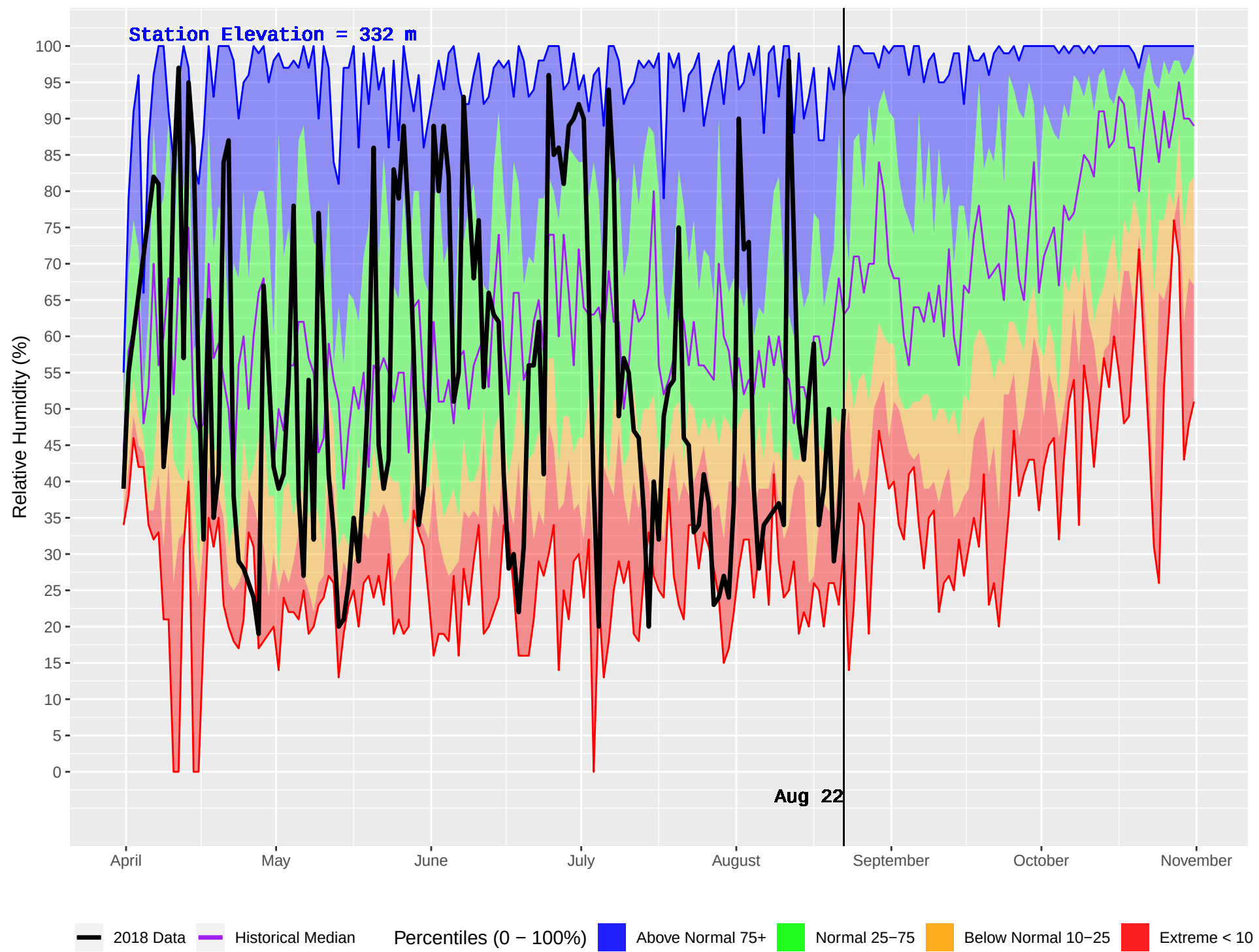
MACHMELL (101) : Historical (1990–2016) and Current (2018) Daily Relative Humidity
