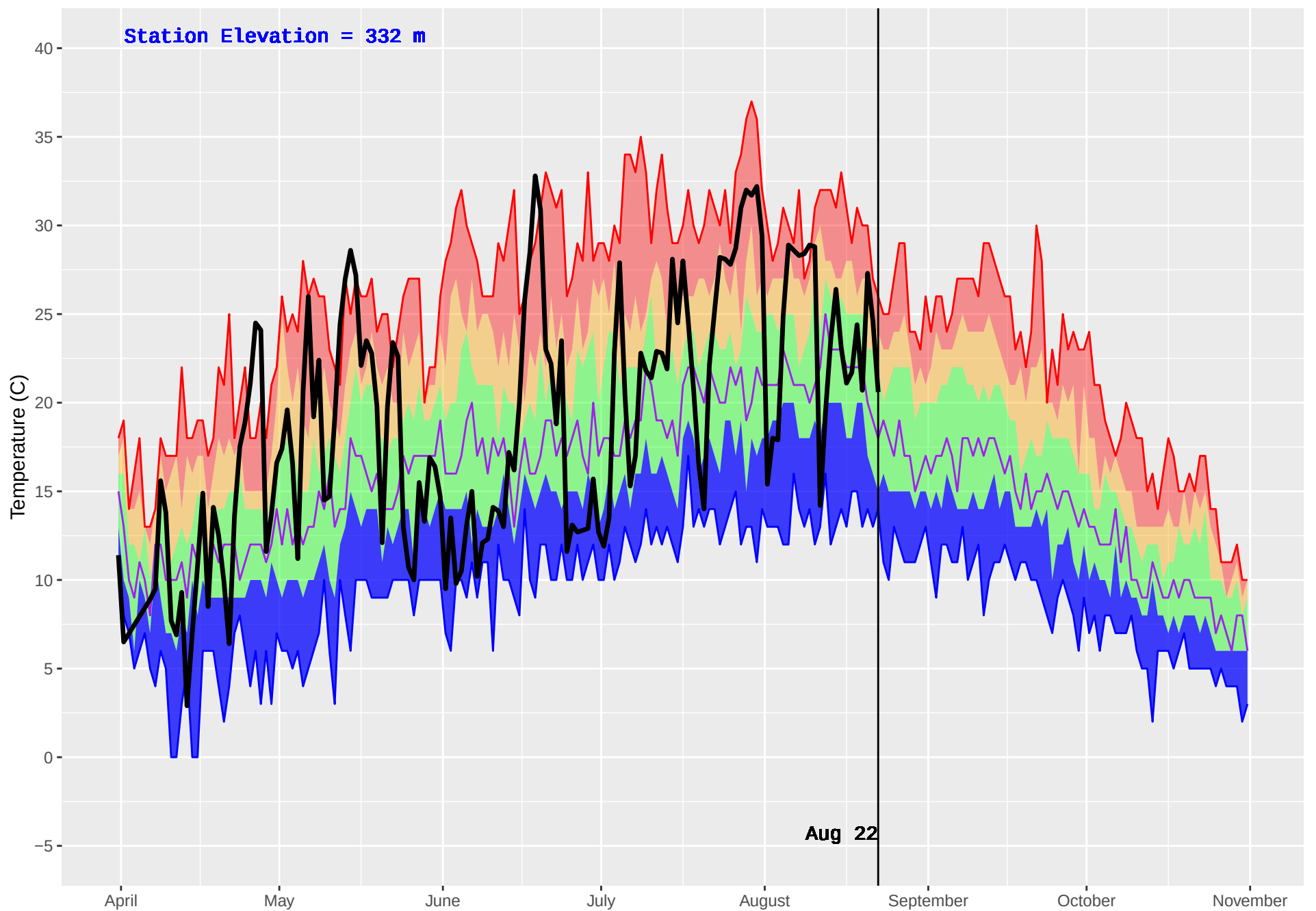
MACHMELL (101) : Historical (1990–2016) and Current (2018) Daily Temperature
