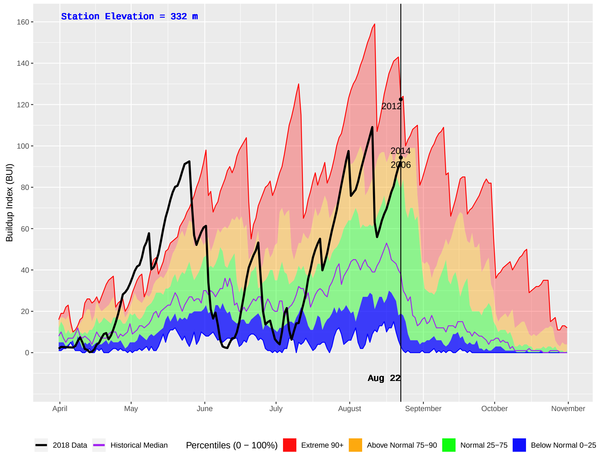
MACHMELL (101) : Historical (1990–2016) and Current (2018) Daily Buildup Index (BUI)
